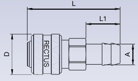
Hose Barb
