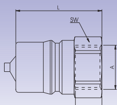
Female Thread
