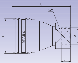
Female Thread
