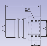
Female Thread
